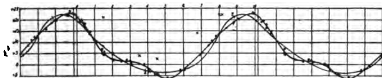
FIGURE 10. Radial Velocity Curve of \zeta Geminorum. The secondary oscillation is probably real
